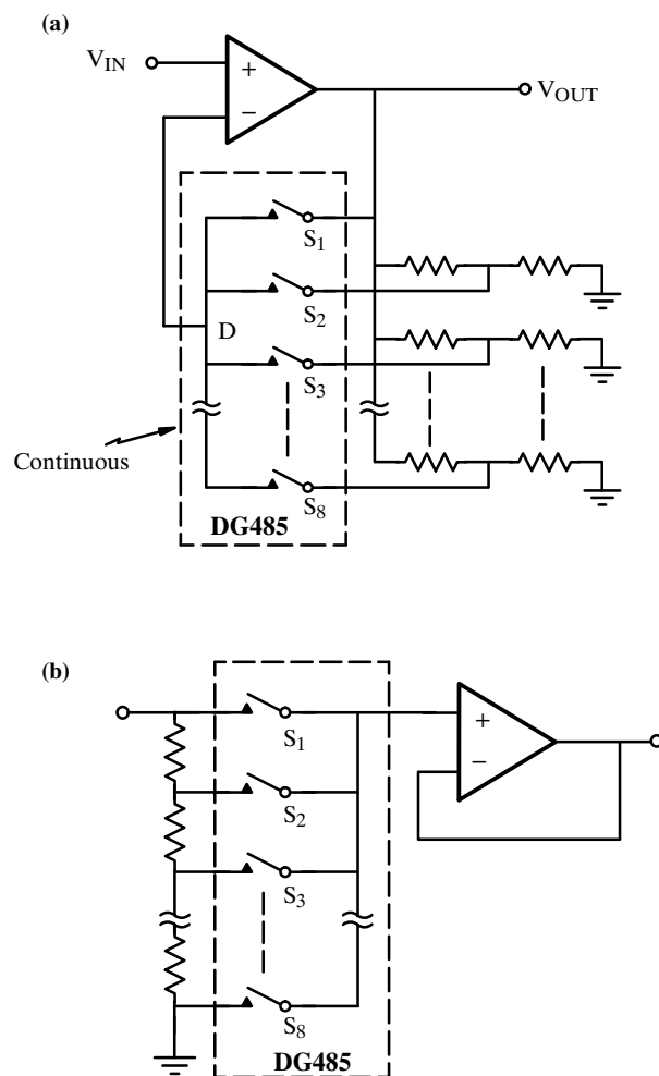
Figure 4. Gain Ranging and Attenuator Circuits
