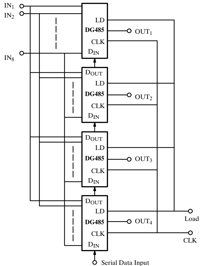
Figure 7. An Eight-by-Ffour Audio Crosspoint
